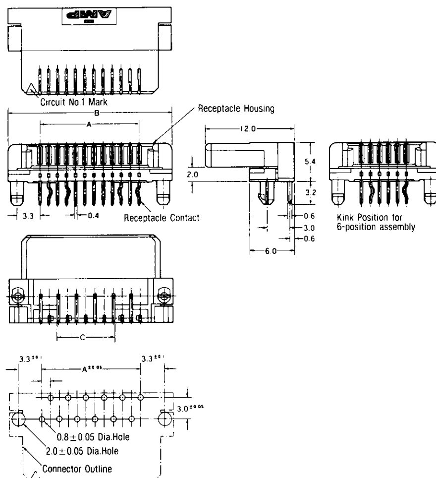
PC Board Layout (Recommended PC Board thickness : 1.6mm)
