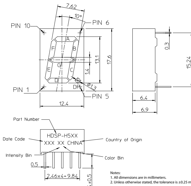
Figure 1 Package Dimension
