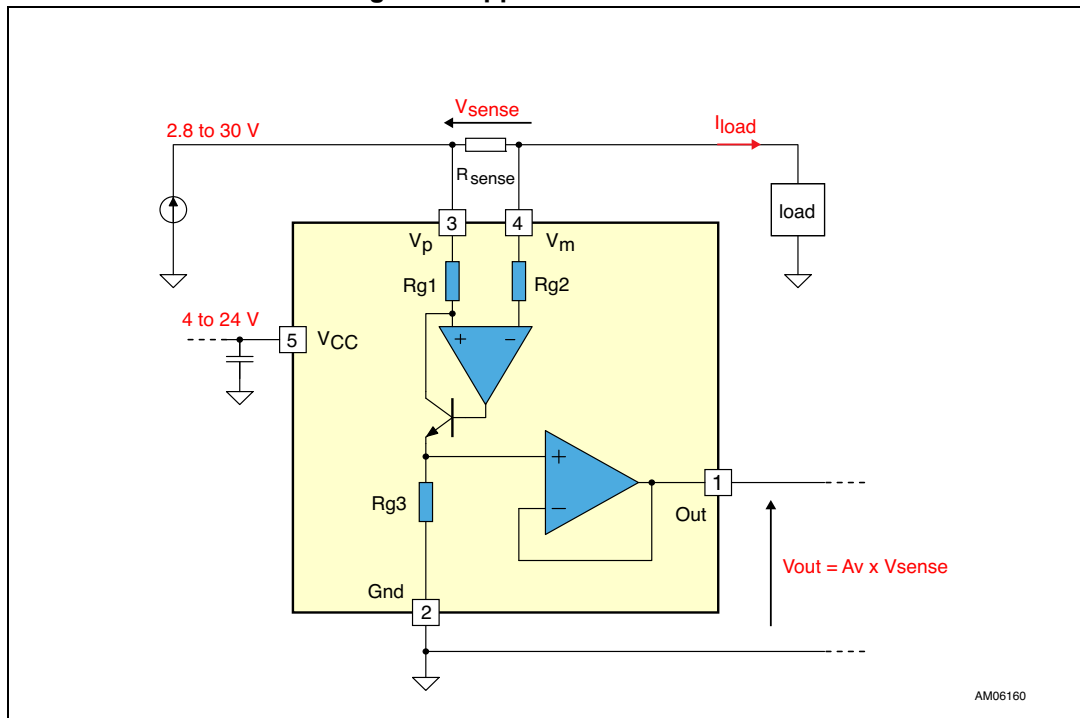
Figure 1. Application schematic
