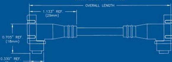
FEMALE RECEPTACLE
