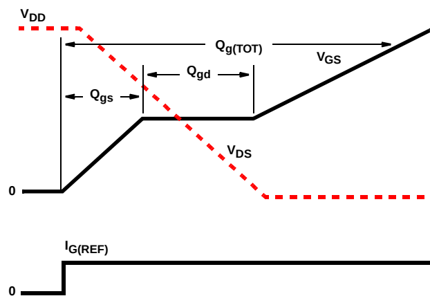
FIGURE 15. GATE CHARGE WAVEFORM
