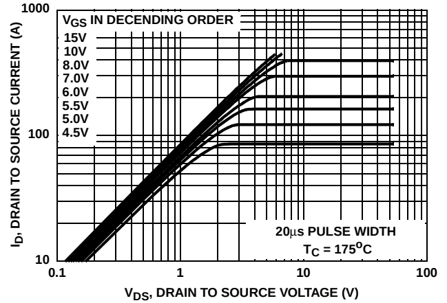
FIGURE 2. OUTPUT CHARACTERISTICS
