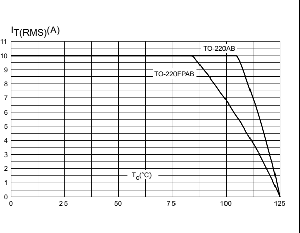
Figure 3. On-state RMS current vs. case temperature (full cycle)
