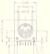
D5-FS 5 Pin PCB mounting DIN socket with EMI / RFI screen. Other pin configurations available. Refer to drawing for details.
