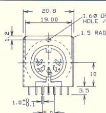
D3 3 Pin right angle PCB mounting DIN socket. 5 Pin versions also available.
