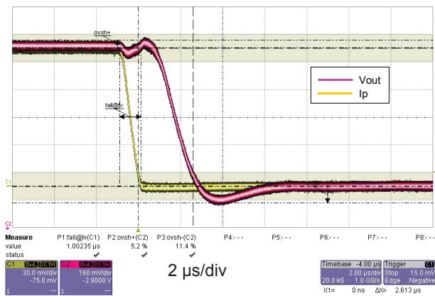
Figure 8: Step response
