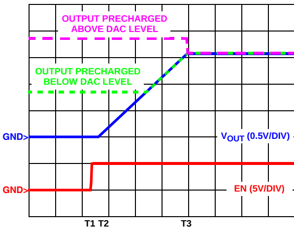
FIGURE 15. SOFT-START WAVEFORMS FOR ISL6313B-BASED MULTI-PHASE CONVERTER
