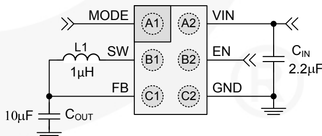
Figure 1. Typical Application
