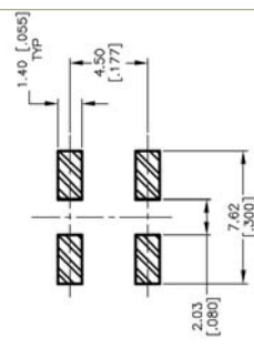
P.C. MOUNTING
