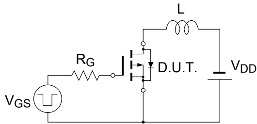
Test Circuit
