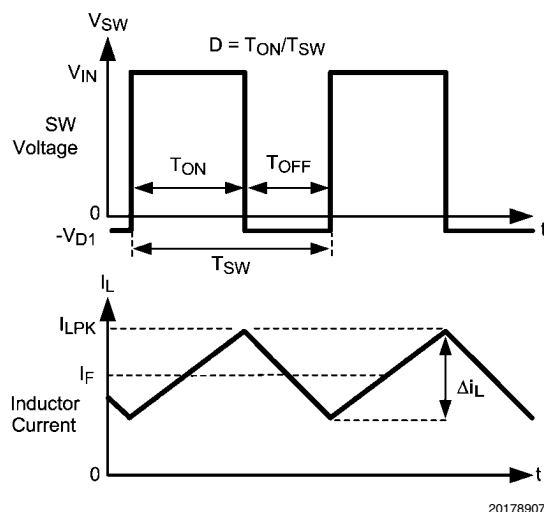
FIGURE 2. SW Pin Voltage and Inductor Current Waveforms of LM3405
