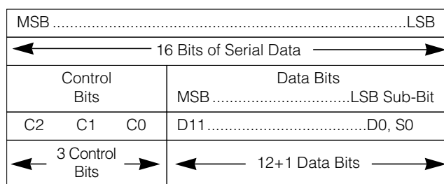
Figure 4. Serial-Data Format
