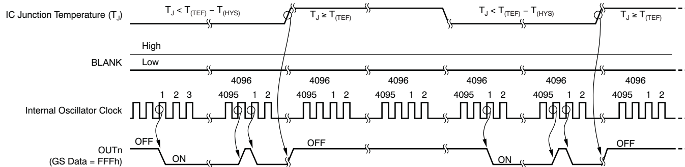
Figure 22. TSD Operation
