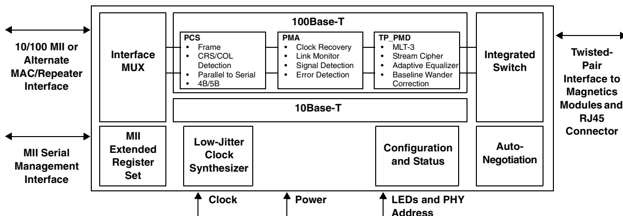
ICS1893CY-10 Block Diagram
