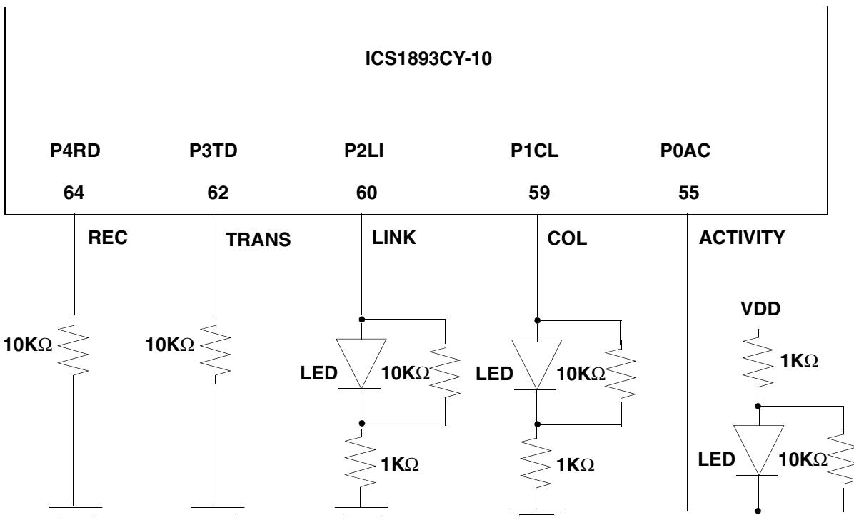
Figure 5-3. ICS1893CY-10 LED - PHY Address
