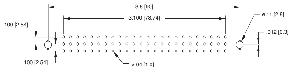
Recommended PCB Layout - Female
