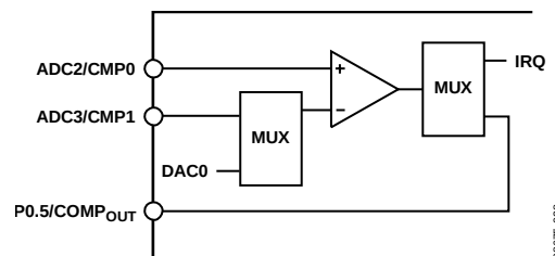
Figure 34. Comparator
