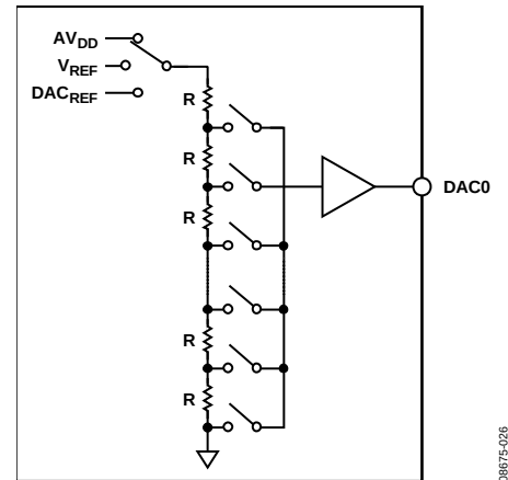
Figure 32. DAC Structure
