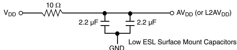
Figure 38. PLL Power Supply Filter Circuit
