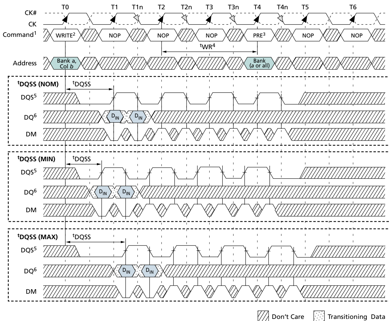
Figure 43: WRITE-to-PRECHARGE – Interrupting
