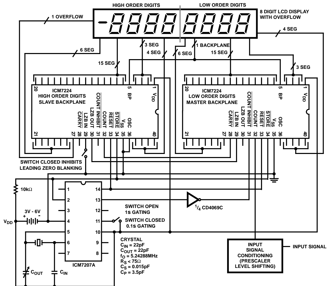
FIGURE 8. EIGHT-DIGIT PRECISION FREQUENCY COUNTER
