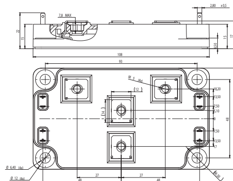
SP6 3-Level
