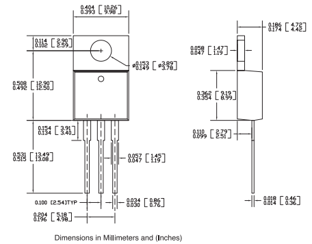
TO-220 3-Lead
