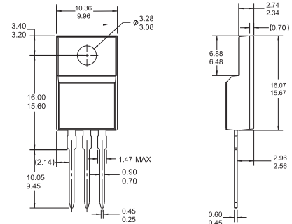
TO-220 [KF]
