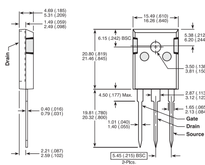
TO-247 3-Lead
