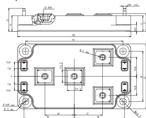
SP6 - 4 outputs
