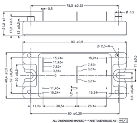
SP6 - 4 outputs
