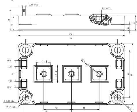
SP6 - 3 outputs
