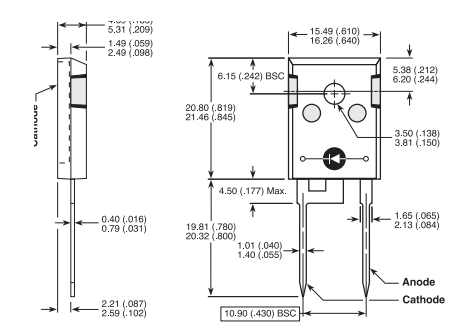
TO-247 2-Lead
