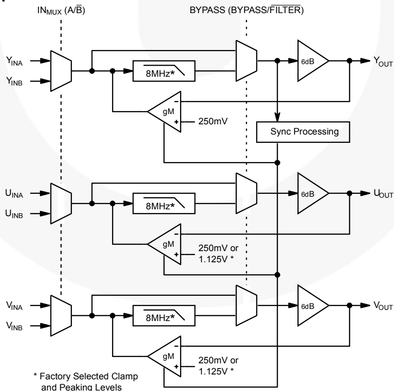
Figure 1. Block Diagram
