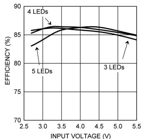
Typical Efficiency (LM3410X)
