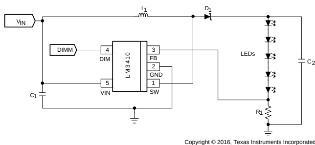
Typical Boost Application Circuit
