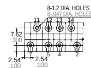
PC board pattern (Copper-side view)
