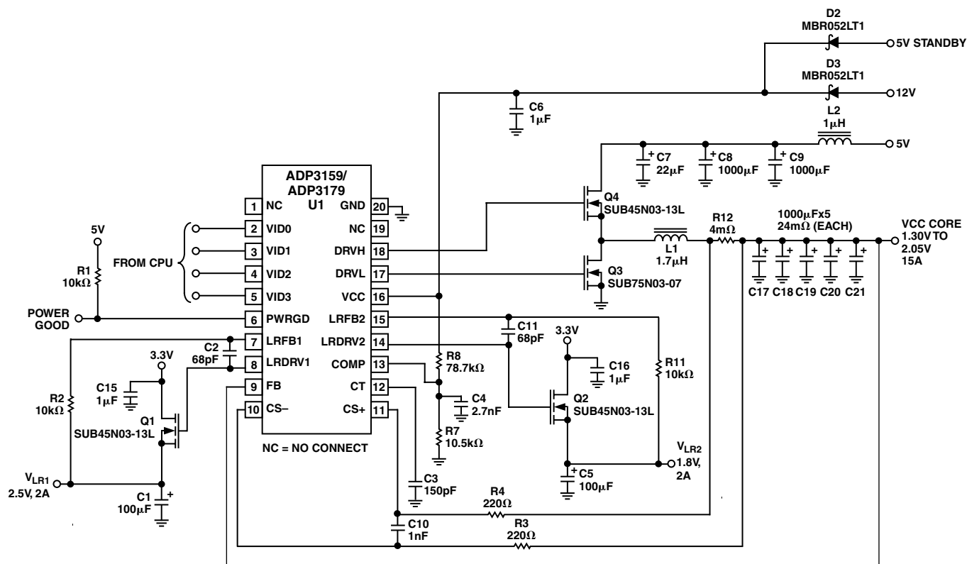
Figure 3. 15 A Pentium III Application Circuit
