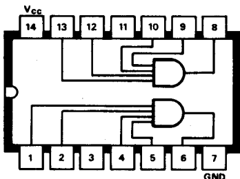
B21 SN74H22N/SN74S22N Dual 4-input NAND gate with open collector output
