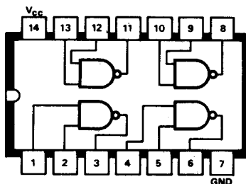
B23 SN7426N Quad 2-input NAND gate with open collector output
