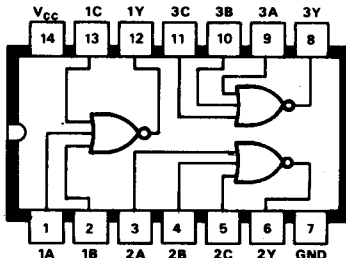
B24 SN7427N Triple 3-input NOR gate
