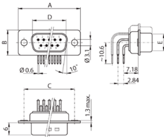
Plug connector
