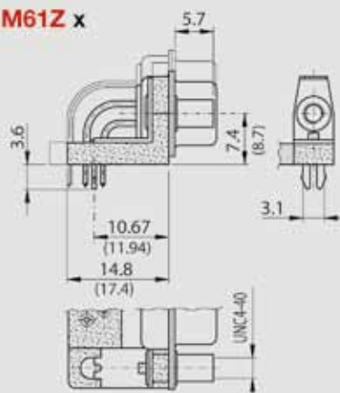
Plastic Bracket with Ground Clip
