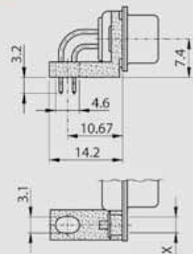
Plastic Bracket
