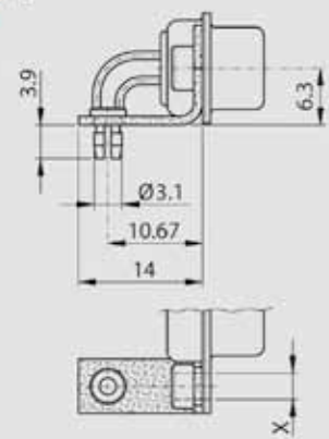
Metal Bracket with P.o.F.
