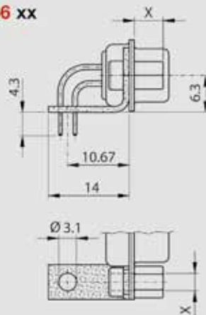
Metal Bracket
