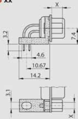
Plastic Bracket
