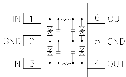
SC-89 (Top View)
