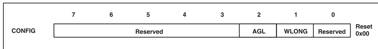
Figure 28: Configuration Register
