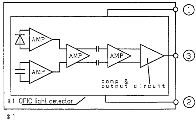
Internal equivalent circuit
