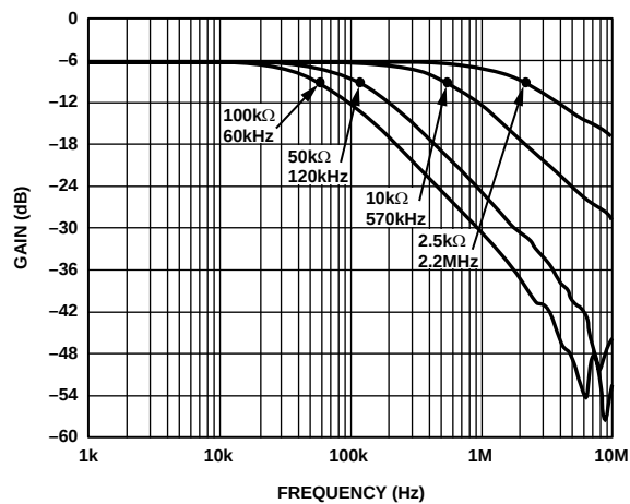
Figure 22. -3 dB Bandwidth @ Code = 0x80
