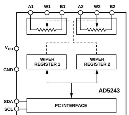
Figure 1. AD5243
