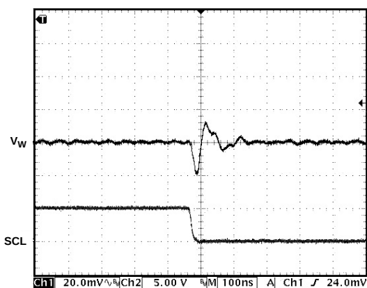
Figure 24. Digital Feedthrough
