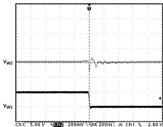
Figure 25. Digital Crosstalk
