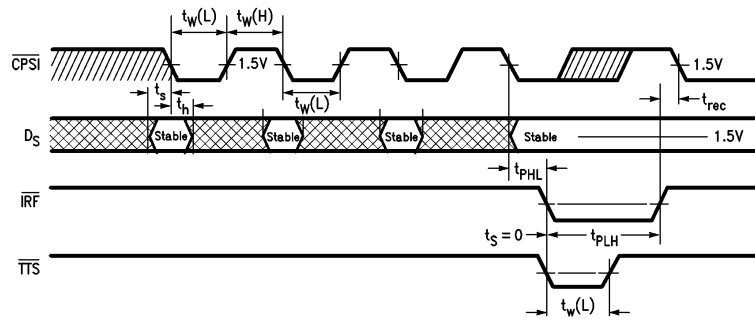
FIGURE 9403A-a. Serial Input, Unexpanded or Master Operation
