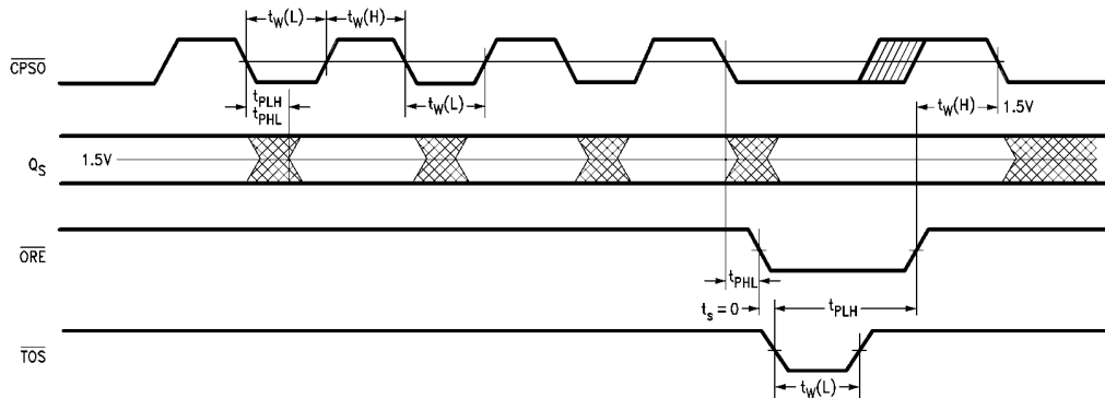
FIGURE 9403A-b. Serial Input, Expanded Slave Operation
