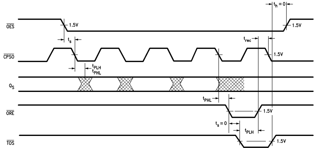
FIGURE 9403A-d. Serial Output, Slave Operation
