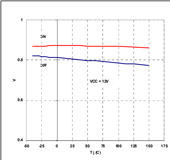
Figure 26. RUN threshold vs T_J
