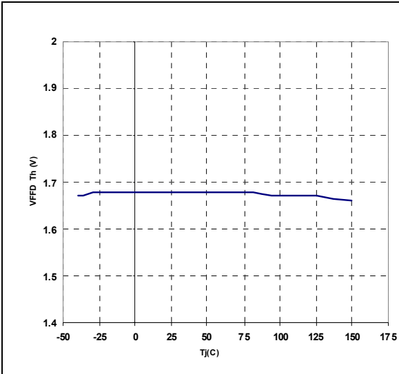
Figure 24. PFC_OK FFD threshold vs T_J
