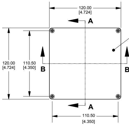
Top View of Assembly
