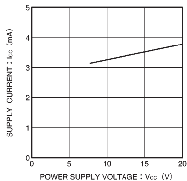
Fig.11 Supply current vs. power supply voltage
