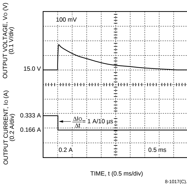
Figure 6. DC025 Dual-Output-Series Typical 15 V Output Voltage Response to a Step Load Change from 50% to 25% of I_{o,max} at V_i = V_{i,nom} and T_c = 25^\circ\text{C}
