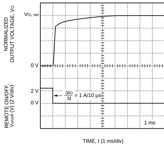
Figure 10. DC025 Dual-Output-Series Typical Output Voltage Rise Time with Remote On/Off at V_i = V_{i, \text{nom}} , I_o = 0.8 (I_{o, \max}) , and T_c = 25^\circ\text{C}
