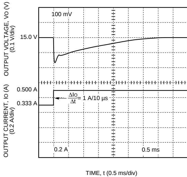
Figure 9. DC025 Dual-Output-Series Typical 15 V Output Voltage Response to a Step Load Change from 50% to 75% of I_{o, \max} at V_i = V_{i, \text{nom}} and T_c = 25^\circ\text{C}
