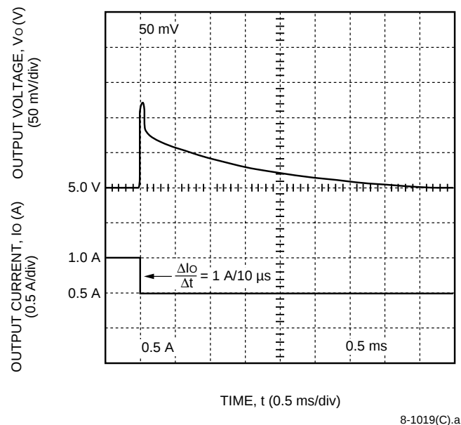
Figure 4. DC025 Dual-Output-Series Typical 5 V Output Voltage Response to a Step Load Change from 50% to 25% of I_{o,max} at V_i = V_{i,nom} and T_c = 25^\circ\text{C}
