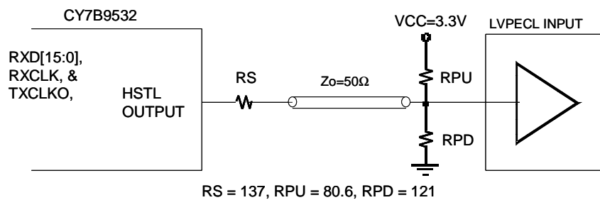
Figure 6. LVPECL Compliant Termination
