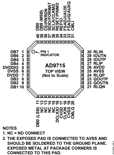
Figure 3. AD9715 Pin Configuration
