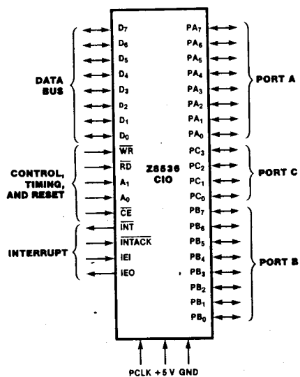
Figure 1. Pin Functions
