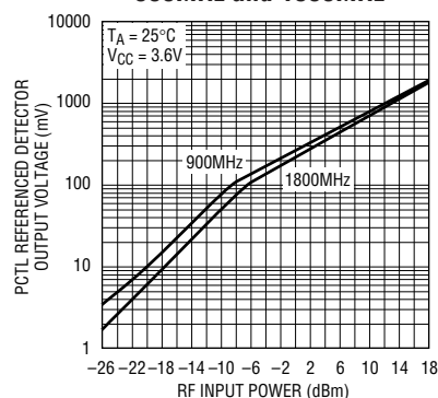
LTC4400-1 Detector Characteristics at 900MHz and 1800MHz
