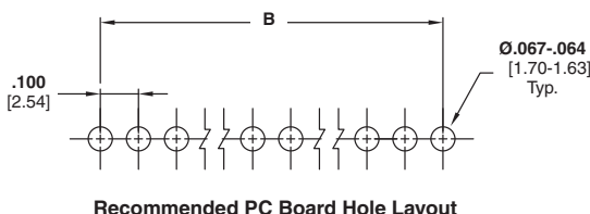
Recommended PC Board Hole Layout
