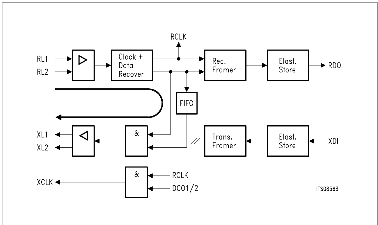
Figure 51 Remote Loop
