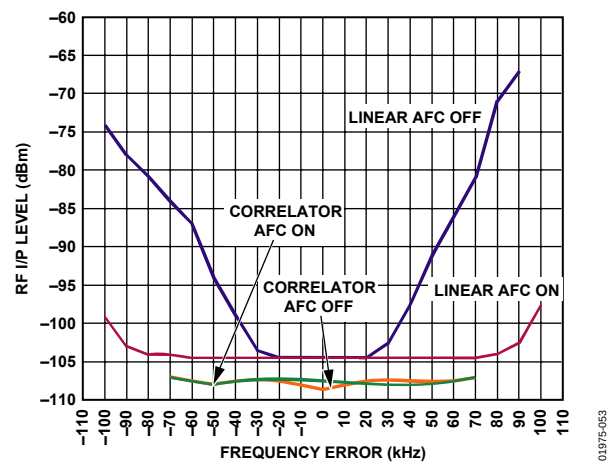
Figure 18. Sensitivity vs. Frequency Error with AFC On/Off
