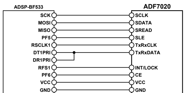
Figure 36. ADSP-BF533 to ADF7020 Connection Diagram
