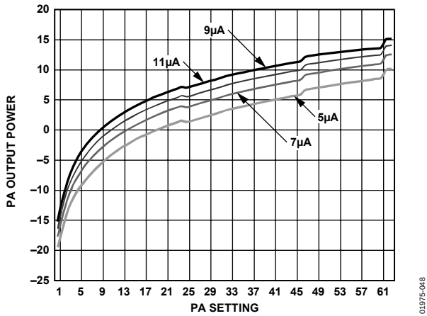
Figure 13. PA Output Power vs. Setting
