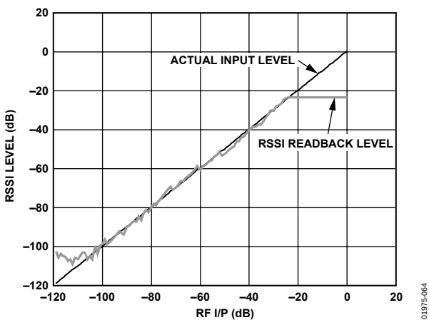
Figure 15. Digital RSSI Readback Linearity
