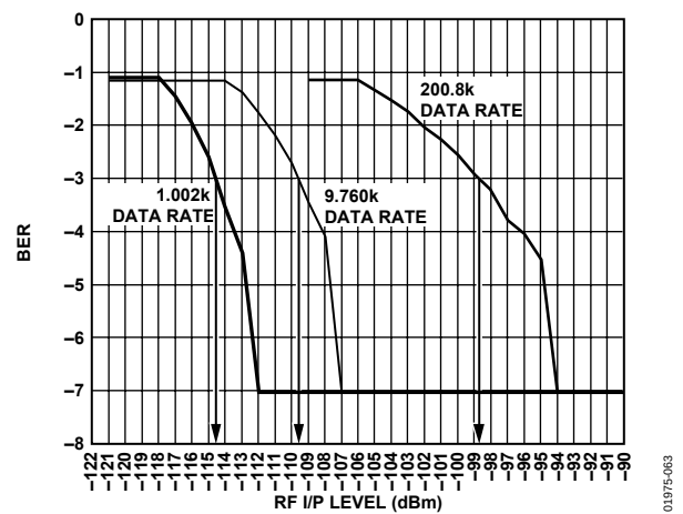
Figure 17. BER vs. Data Rate (Combined Matching Network) Separate LNA and PA Matching Paths Typically Improve Performance by 2 dB
