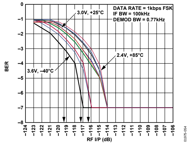
Figure 16. Sensitivity vs. VDD and Temperature
