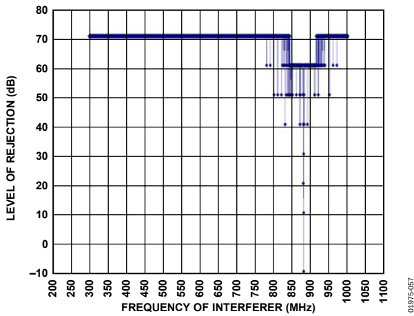
Figure 14. Wideband Interference Rejection; Wanted Signal (880 MHz) at 3 dB above Sensitivity Point Interferer = FM Jammer (9.76 kbps, 10 kHz Deviation)
