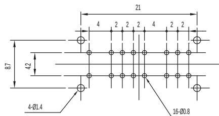
PIERCING PLAN
