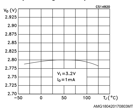
Figure 4: Output voltage vs temperature V_O = 2.8\text{ V}
