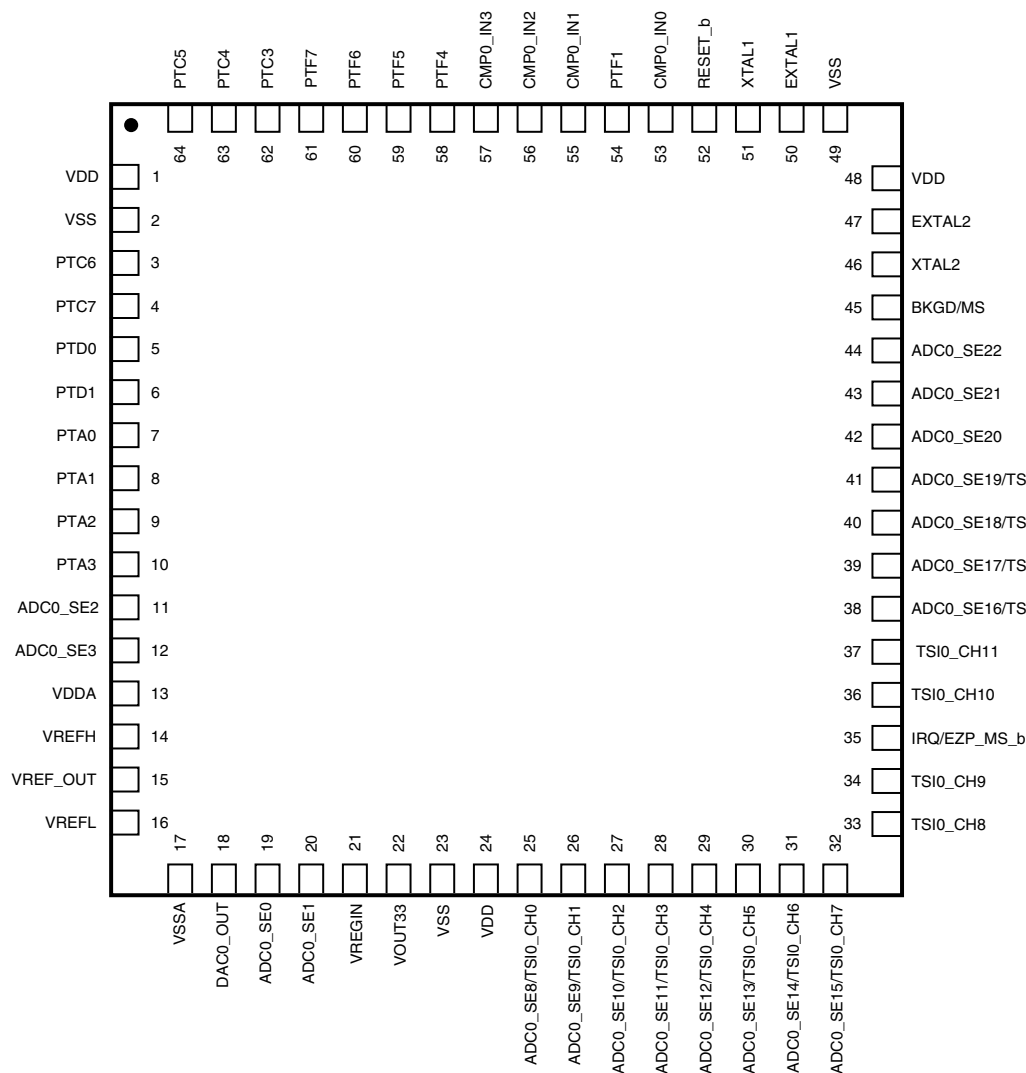
Figure 18. 64-pin Laminate QFN (pinout identical for 64-pin LQFP)
