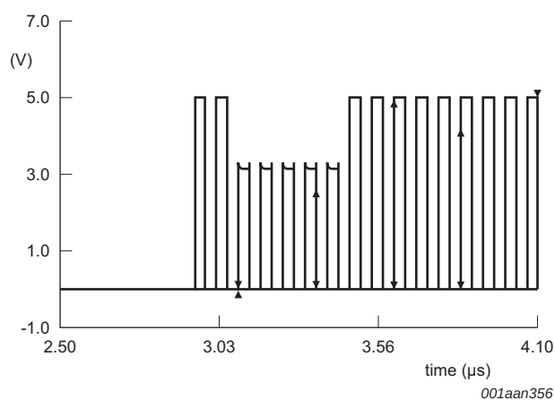
Fig 26. Example 1: overshoot_t1 = 2d; overshoot_t2 = 5d.
