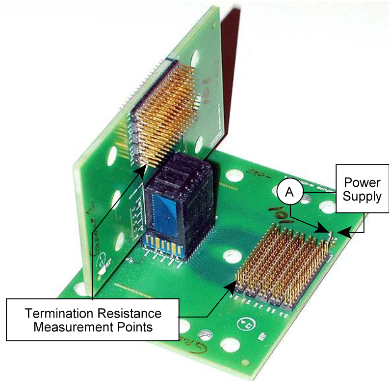
Figure 3 Low Level Contact Resistance Measurement Points (Circuit)
