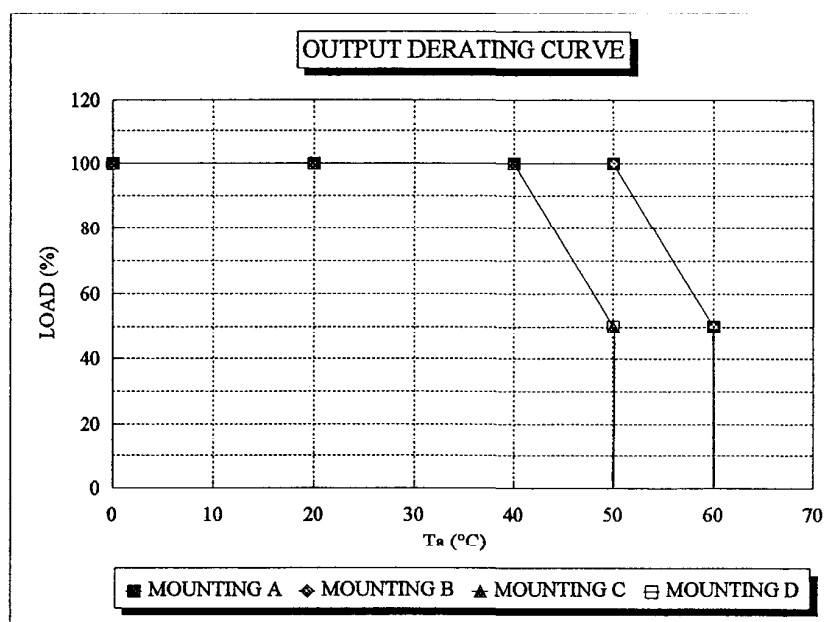
MOUNTING : A
